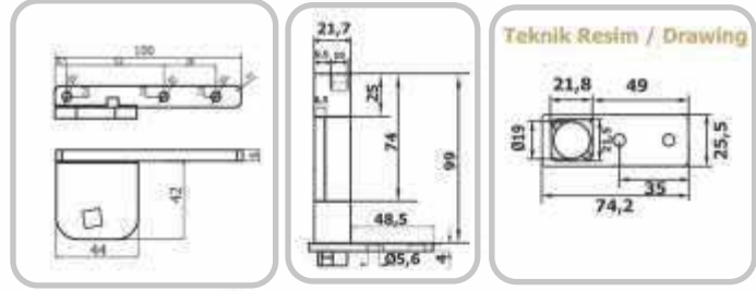
İ-804-06 (Sağ/Right) / İ-804-07 (Sol/Left) YAYLI YAN MENTEŞE SIDE SPRINGED HINGE
